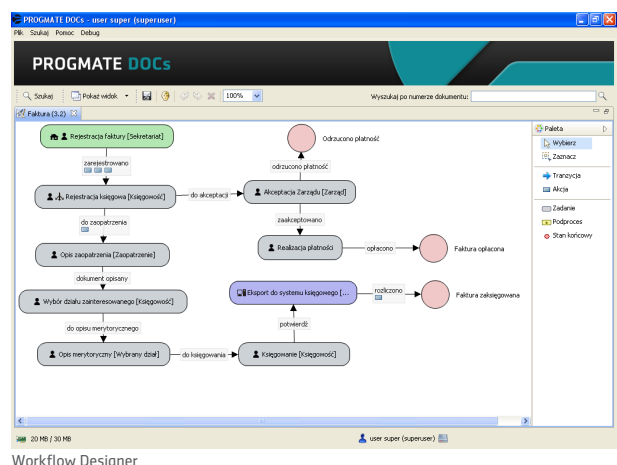
Workflow Designer
